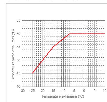
PUD-SWM80VAA / PUD-SWM100/120V/YAA
