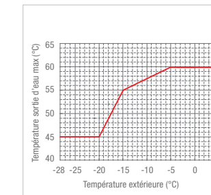
PUZ-HWM140VHA
