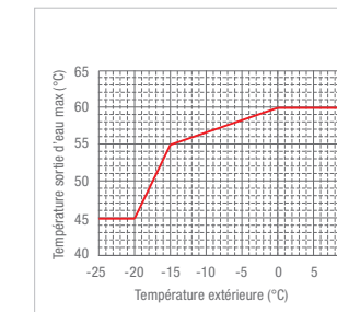
PUZ-WM112VAA
